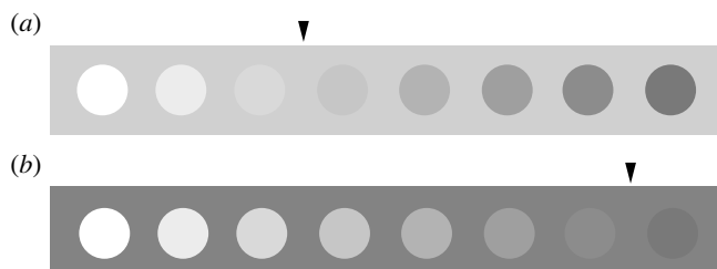
Figure 2. Effect of achromatic background contrast on brightness discrimination. Evidence from humans suggests that stimuli are easiest to discriminate when placed on a background with low brightness contrast [37,54]. We can demonstrate this effect using equally spaced achromatic stimuli on a light grey (a) and dark grey (b) background. The arrows mark the brightness of the background relative to the series of stimuli. Stimuli that are closer in brightness to each background are more easily discriminable, and this effect is most pronounced when the background has an intermediate brightness to the two stimuli. This effect is apparent with colour stimuli, as well, but because digital displays are highly variable, we opt here to show only the achromatic version of this effect.
